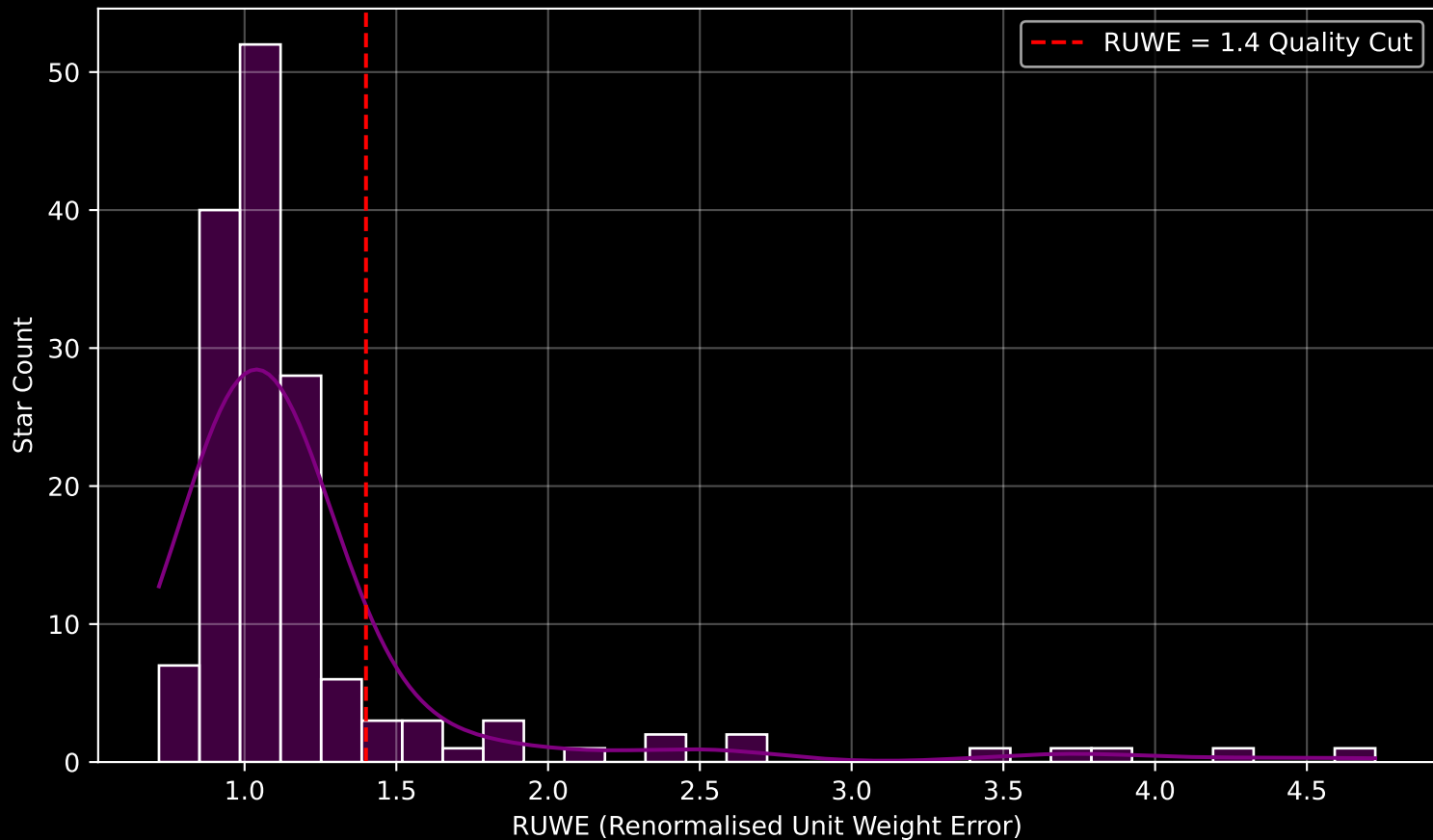
GAPOGEE DR17 Field [278-27-O_TESS] RUWE Distribution (n= 153)
