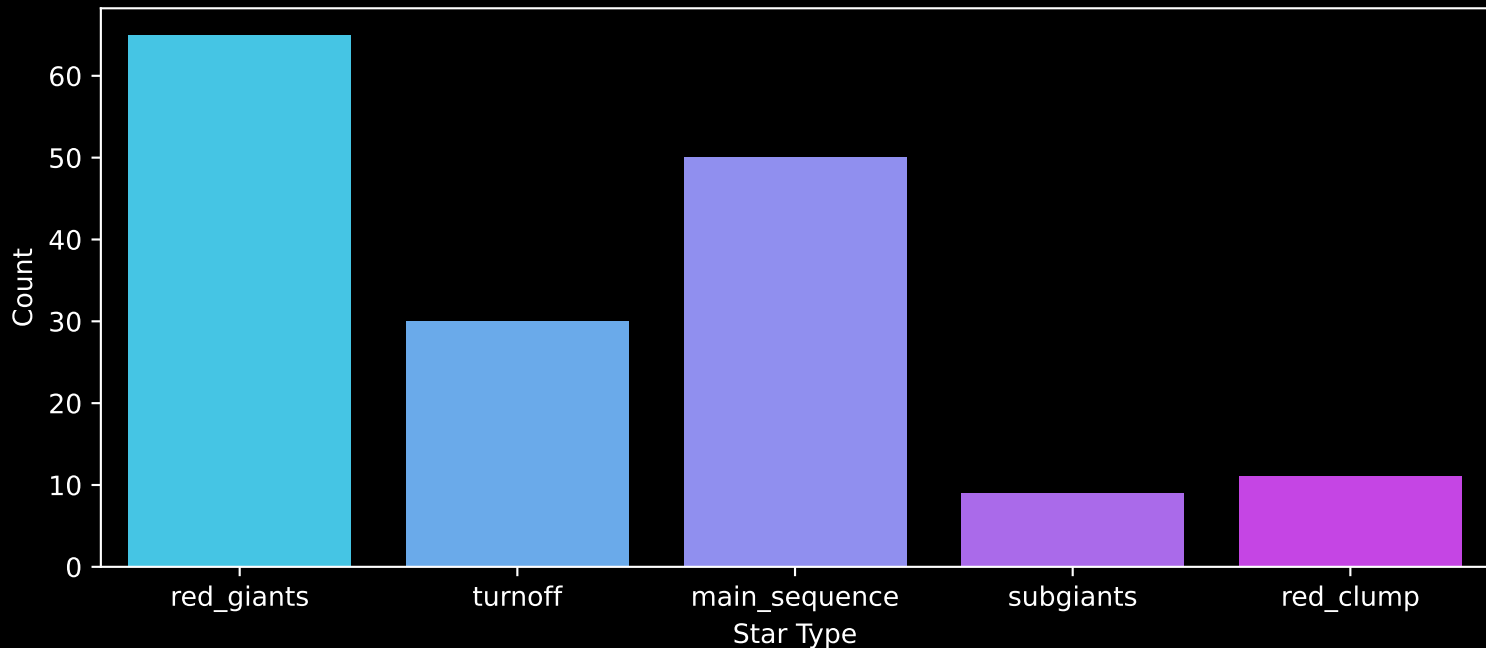
APOGEE DR17 Field: [278-27-O_TESS] Count plot of Star Type
