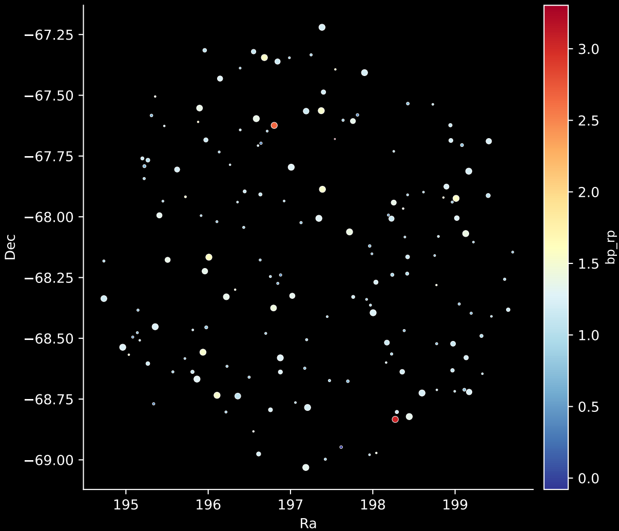
APOGEE DR17 Field: [278-27-O_TESS] Stars: 165
