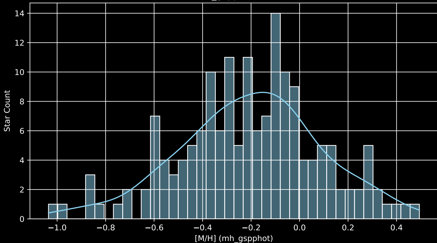
APOGEE DR17 Field: [278-27-O_TESS [M/H] (mh_gspphot) (n= 164)
