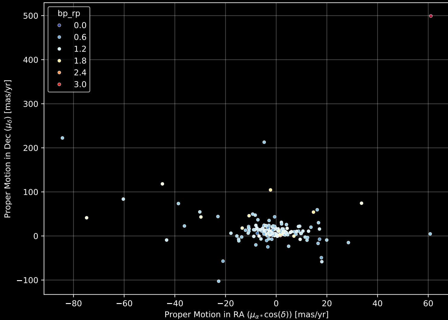
APOGEE DR17 Field: [278-27-O_TESS] Proper Motion Diagram (n= 165)
