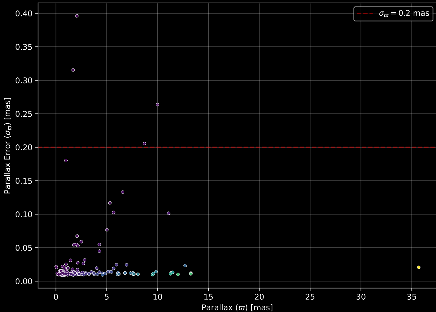
APOGEE DR17 Field: [278-27-O_TESS] Parallax Quality (n= 165)
